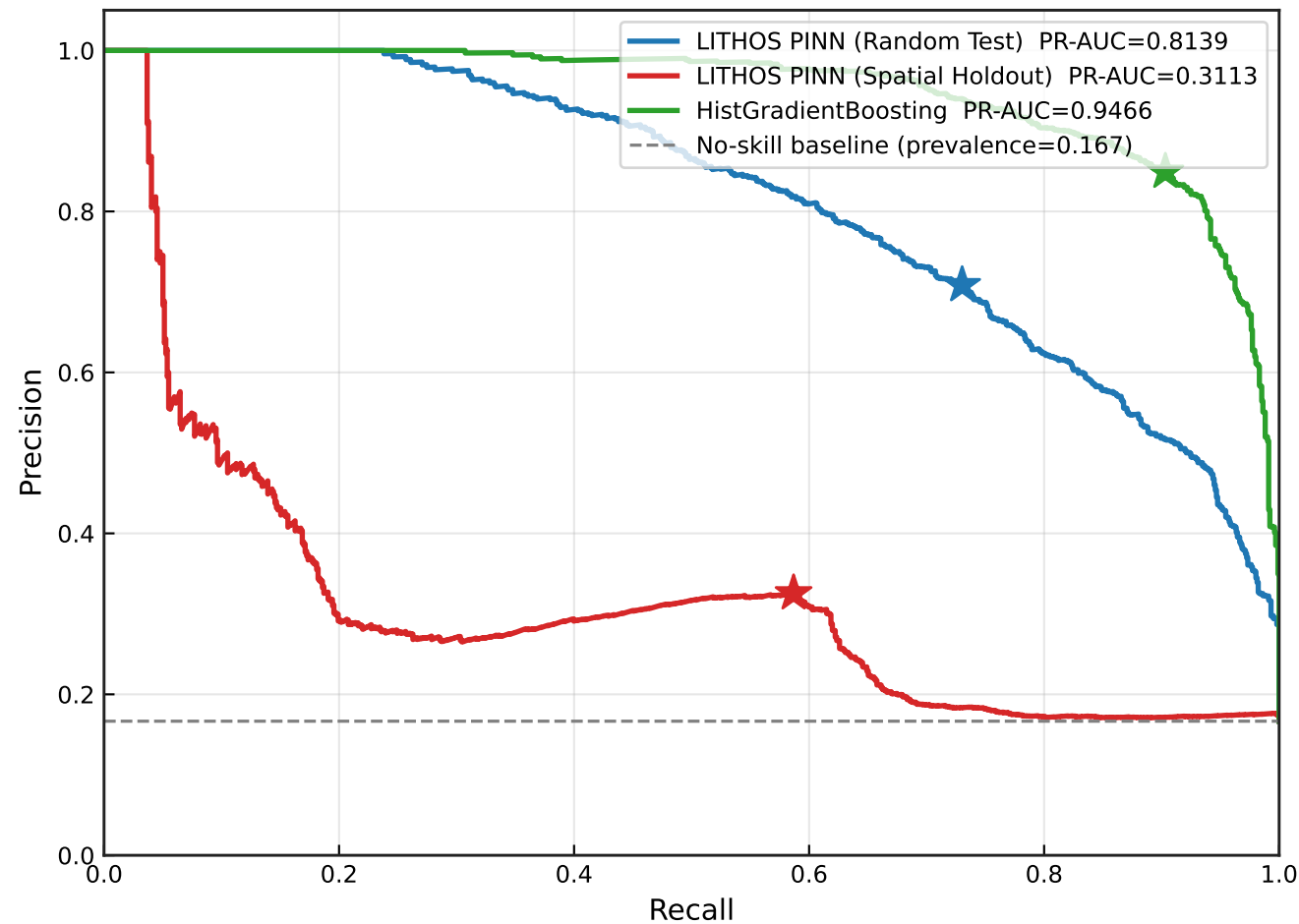
Precision-Recall Curve (* = F1-optimal threshold)
