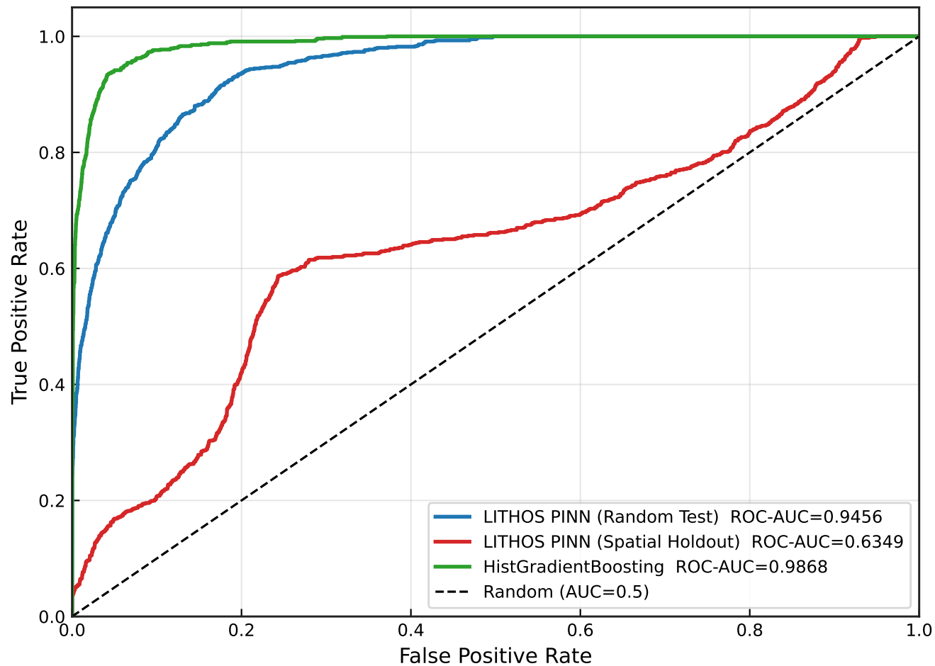
ROC Curve (reference only; PR-AUC is primary)
